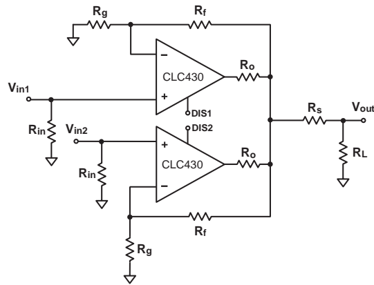
Fig. 5 Output Connection
